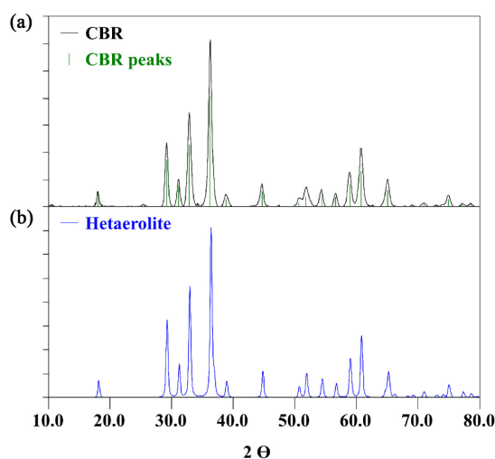
Figure 1. X-ray diffractograms of the (a) CBR material and (b) hetaerolite mineral (chemical formula: \text{ZnMn}_2\text{O}_4 ).
