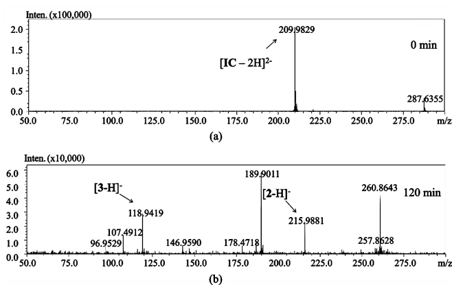
Figure 4. Mass spectra of two aliquots collected at the following reaction times: (a) 0 min; (b) 120 min. The reaction process refers to the degradation of Indigo Carmine induced by the CBR/H 2 O 2 system in an aqueous solution.
