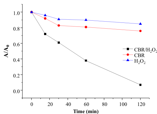
Figure 3. Relative absorbance ( A/A_0 ) of Indigo Carmine solutions monitored during exposure to Fenton-like (CBR/H 2 O 2 ) and controls (CBR and H 2 O 2 ) systems.
