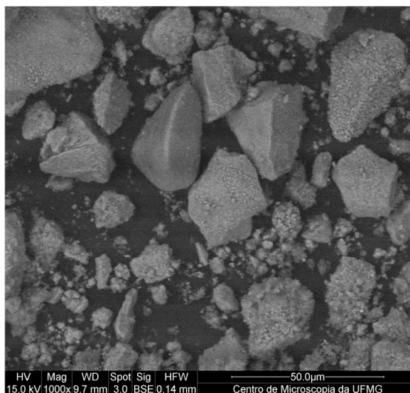
Figure 2. Scanning electron microscopy (SEM) image of the CBR material.
